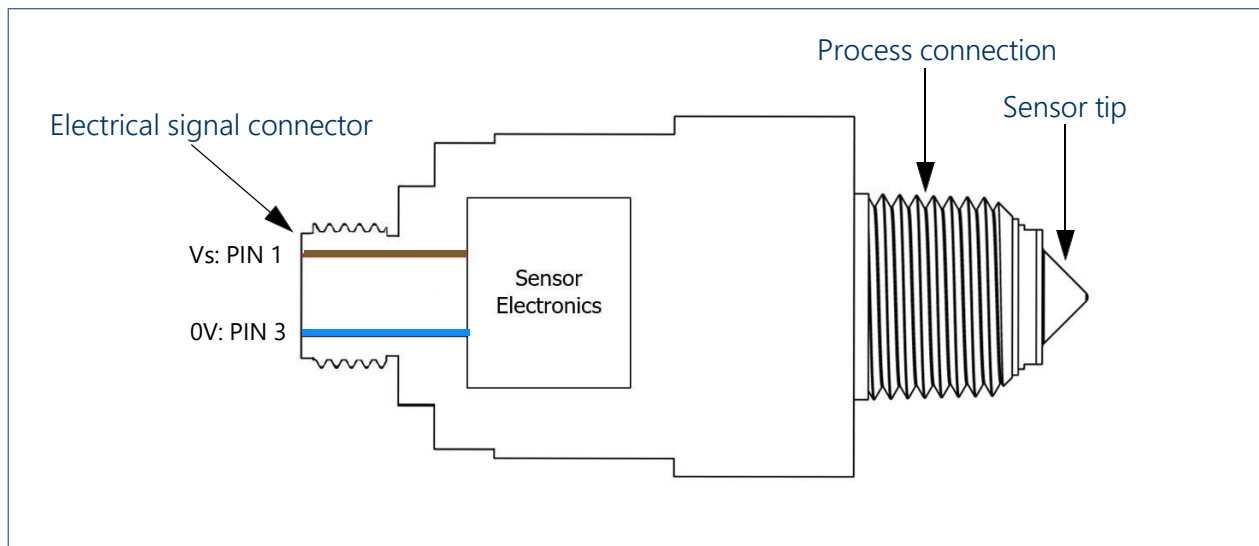
Figure 1. Internal structure
