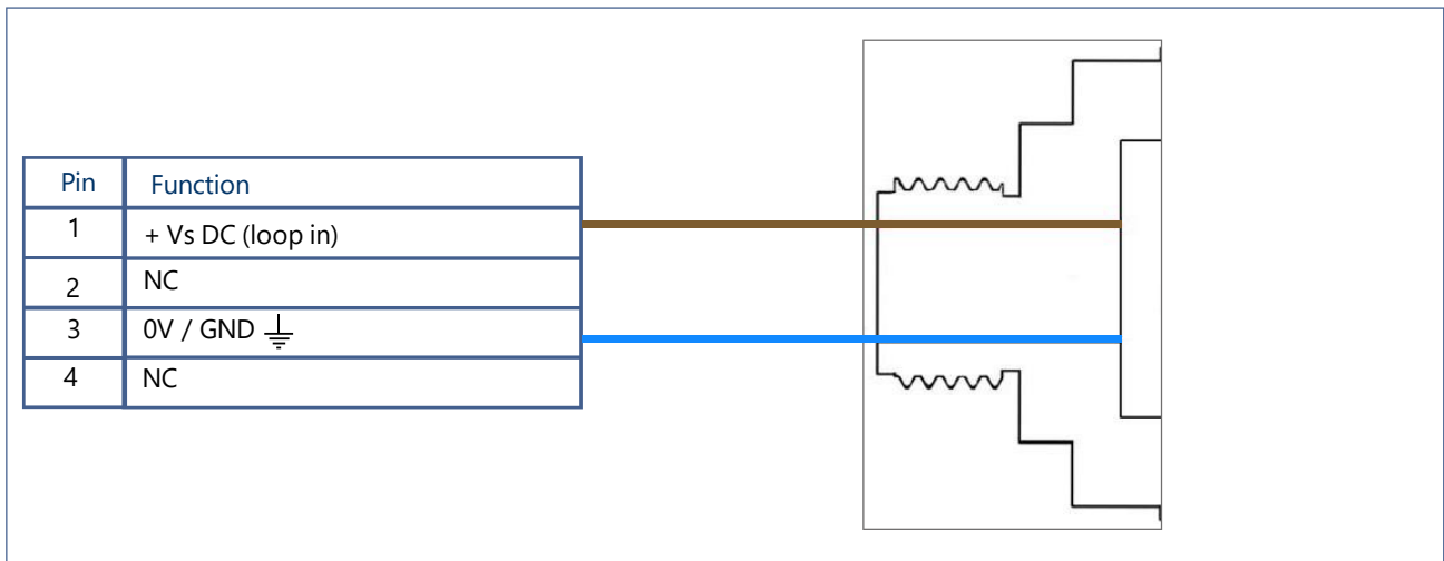
Figure 6. Pin connections
